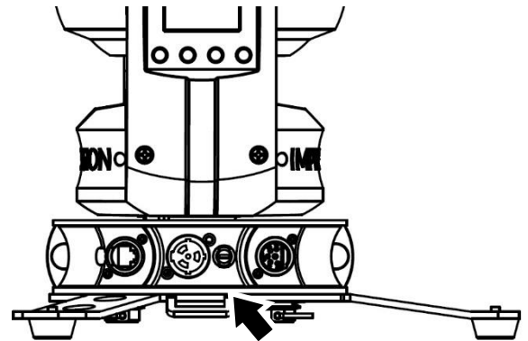
Figure 7. Main fuseholder
