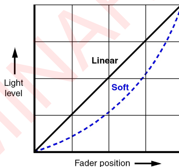
Figure 1. Dimming curves
