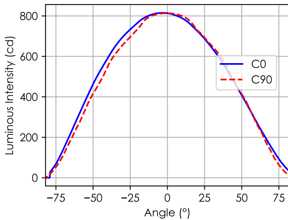
Figure 9: Polar and cartesian light intensity distributions. Plate Blue
