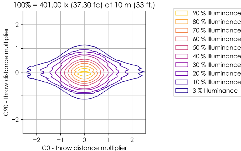
Figure 4: Iso-illuminance diagram of projected beam. Full All dist. from origin = throw dist. x throw dist. multiplier
