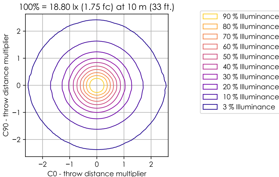
Figure 8: Iso-illuminance diagram of projected beam. Plate Green dist. from origin = throw dist. x throw dist. multiplier
