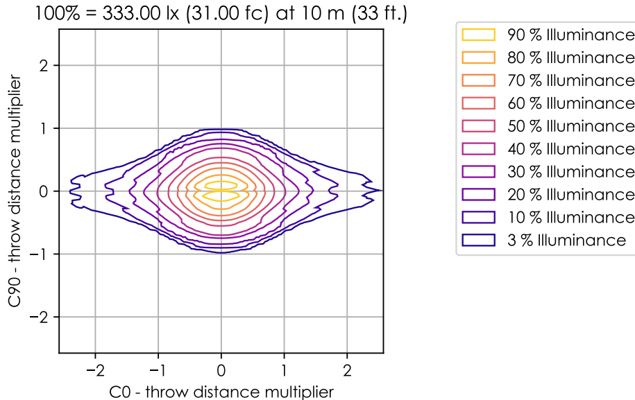
Figure 2: Iso-illuminance diagram of projected beam. Beam dist. from origin = throw dist. x throw dist. multiplier
