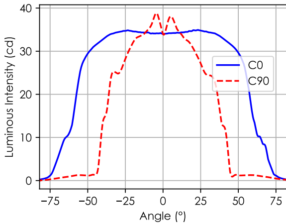
Figure 1: Polar and cartesian light intensity distributions. Beam
