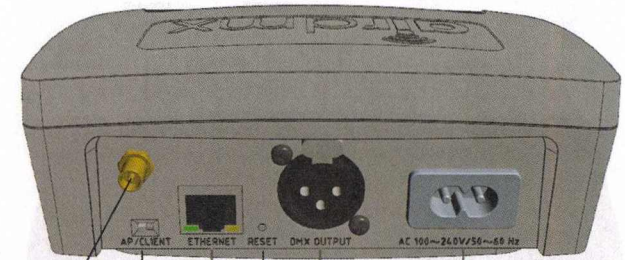
Antenna Port AP/Client Switch Ethernet Reset Button DMX Output Power In
