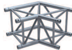
F44C22 2 way 120 degree corner 19.7 in.
